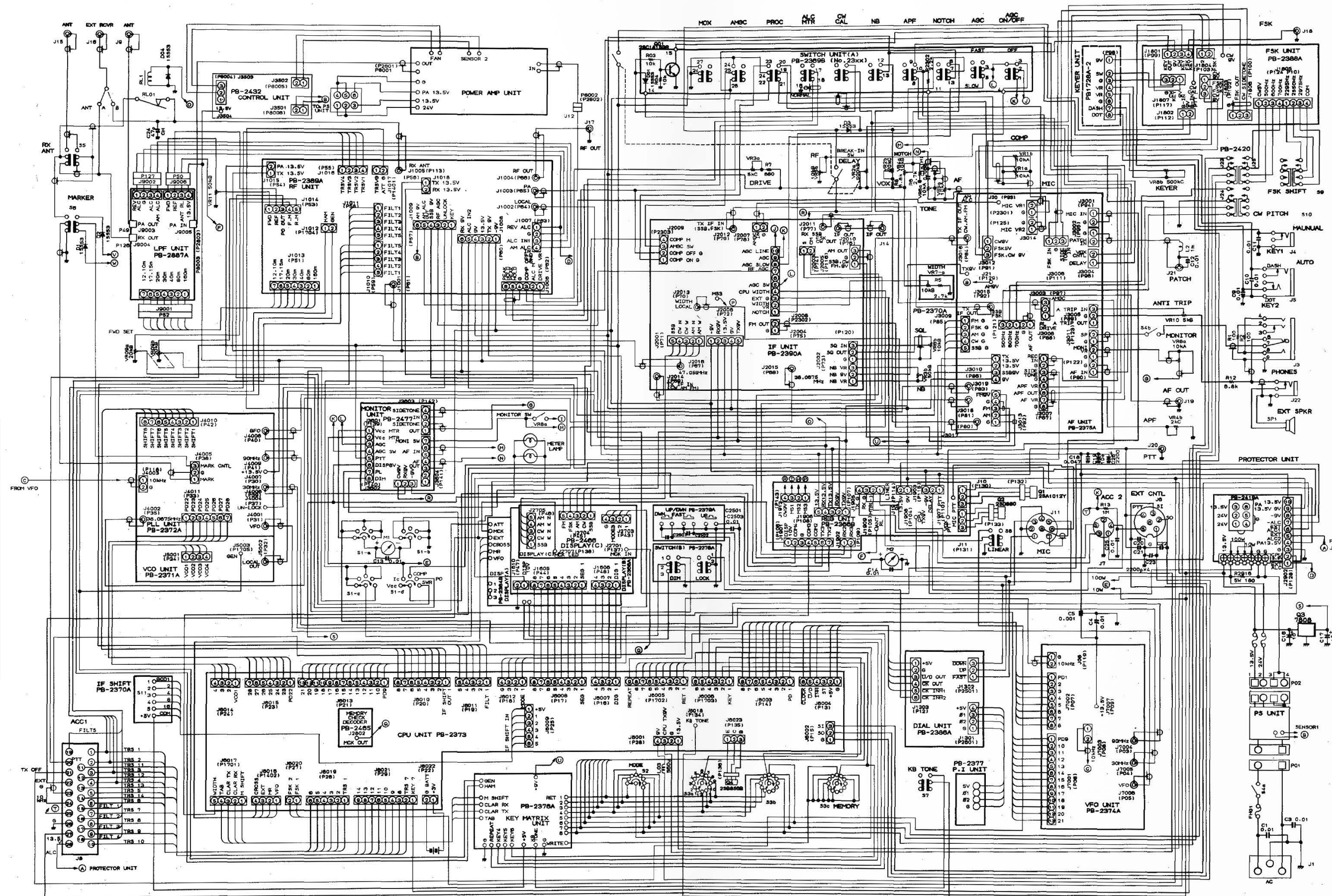
FT-980 CONNECTION DIAGRAM
